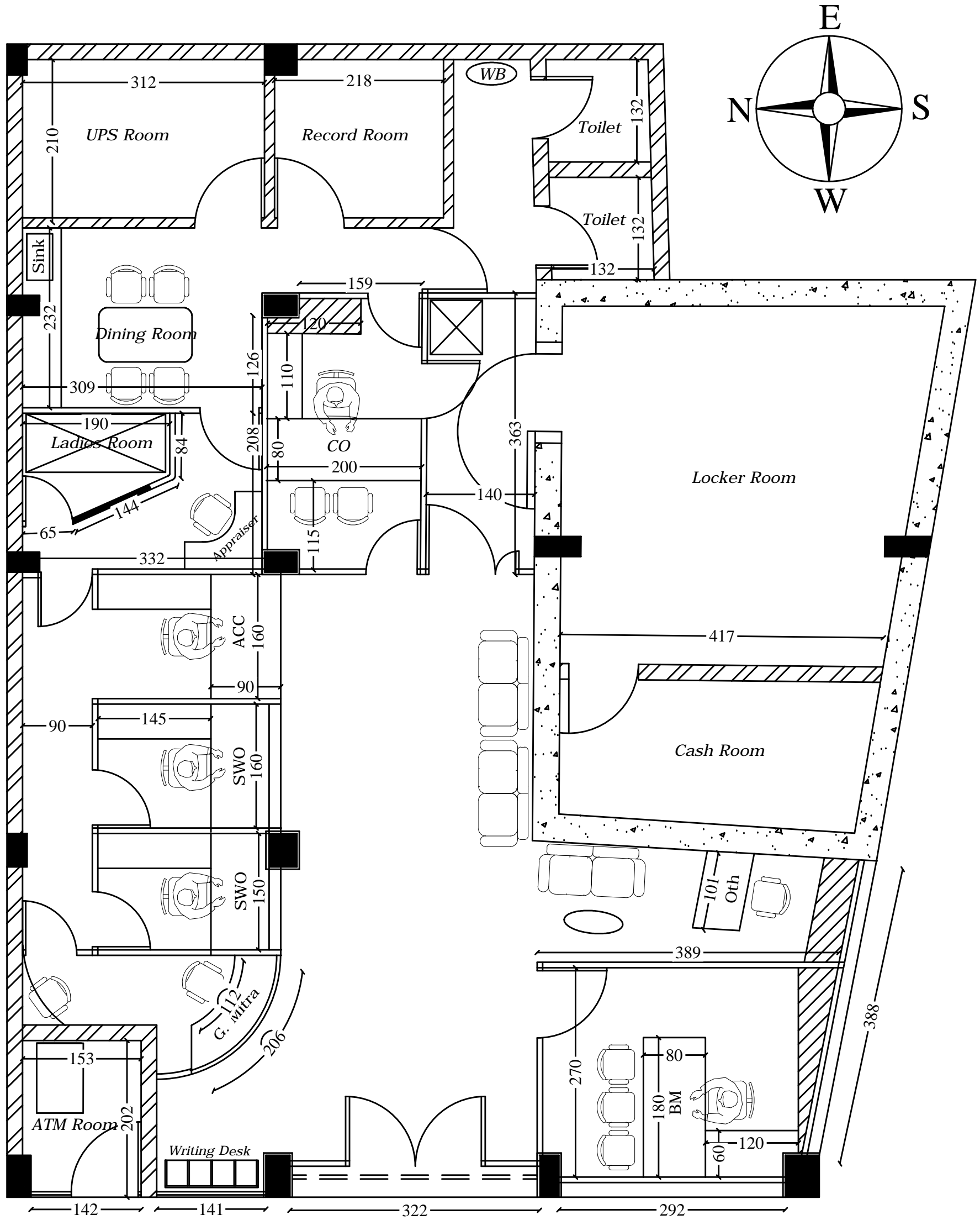
SBI OTTUPARA BRANCH PROPOSED LAYOUT
